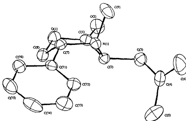
Figure 1. X-Ray structure of morpholinone 11 (crystallographic numbering).
